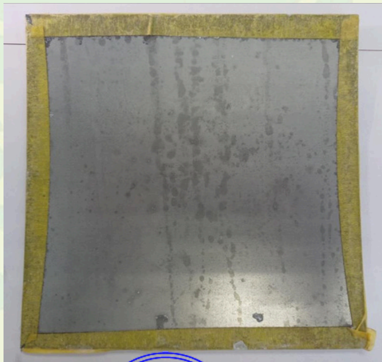
Photo 1.3: Metal plate after NSS 1000 hours (Back view).
